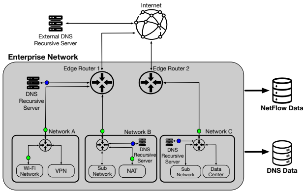
Fig. 1: An abstract representation of an enterprise network with multiple NetFlow (green) and DNS sensors (blue). Large-scale data collection often has issues like data duplication, clock skew, and data loss.
