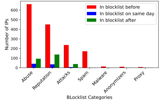
Fig. 7: Orphan IP distribution in our data by malicious category, and relative to the time of their first appearance on blocklists.
