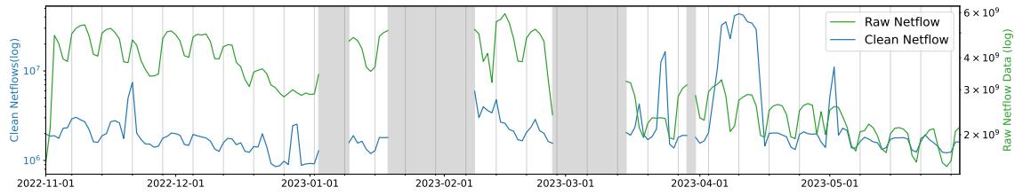
Fig. 2: Volume of raw (green line, right y-axis) and cleaned (blue line, left y-axis) NetFlow per day. The data volume follows an organic cyclic pattern of increasing from the beginning of the week, reaching a peak during the middle of the week, and falling towards the end of the week.
