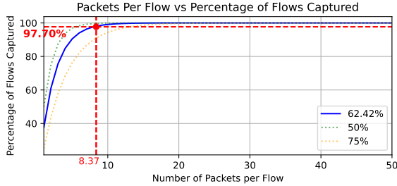
Fig. 3: Results of our statistics-based simulation showing the number of flows that would be recorded/unrecorded ( i.e. , no. packet picked up by a NetFlow sensor) for three levels of packet loss as a function of flow size. Intuitively, flows with more packets are more likely to be recorded.
