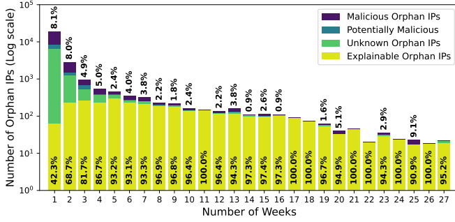
Fig. 8: Orphan IP Persistence. The percentage on the bottom of the bar indicates the percentage of explainable orphan IPs, and the percentage on top of the bar indicates the percentage of malicious orphan IPs in that week.
