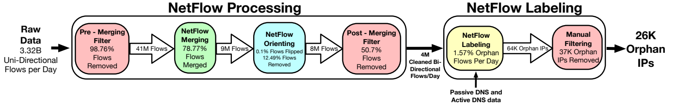
Fig. 4: We employ a two-step process to identify orphan flows. In the first step, NetFlow processing, raw NetFlow data is filtered and merged into bidirectional flows. In the second step, NetFlow labeling, diverse DNS datasets are used to identify orphan flows within the processed bidirectional flows.
