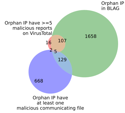
Fig. 6: Venn diagram of malicious and potentially malicious orphan IPs found using VirusTotal, BLAG, and malicious communicating files.
